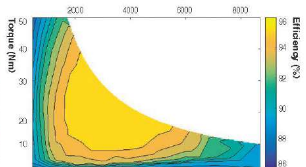
Efficiency/Loss Map
